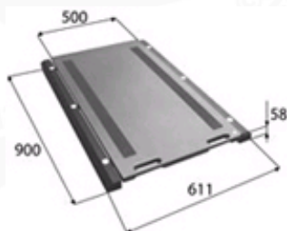
WWSD: Abmessungen in mm.
