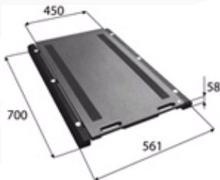
WWSE: Abmessungen in mm.
