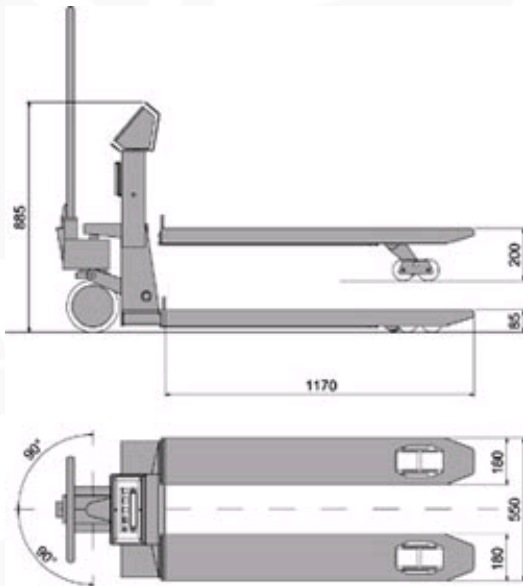
TPWX: Abmessungen in mm.
